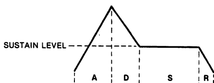
Figure 11-7. ADSR Phases
