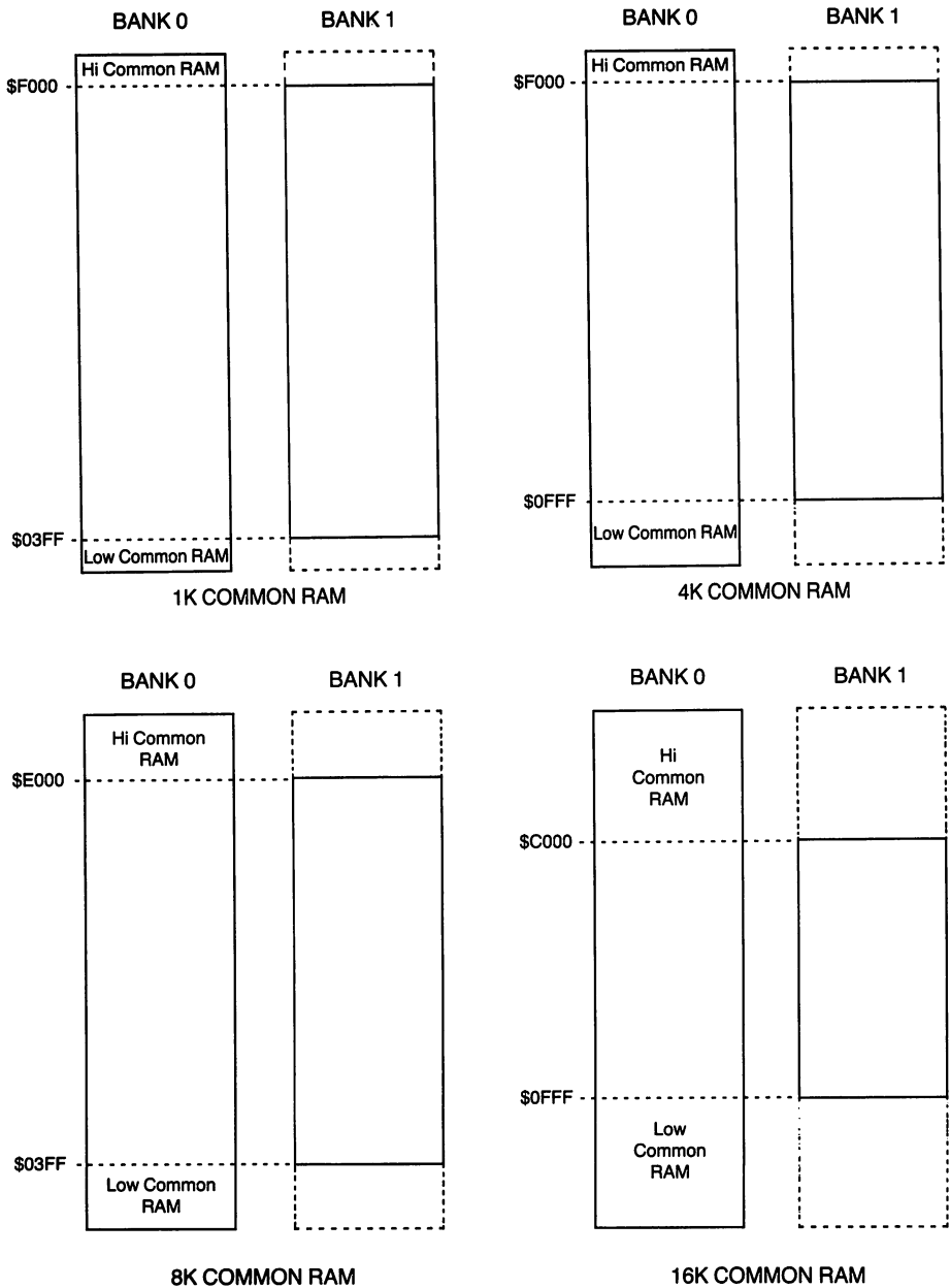
Figure 13-8. Common RAM
