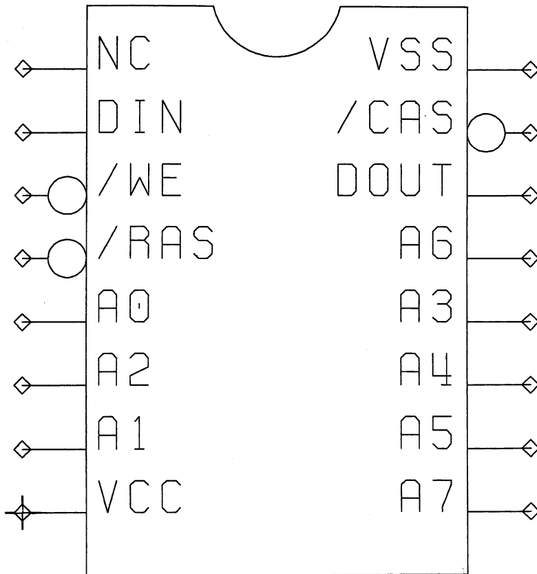
Figure 16-23. The 4164 Chip
