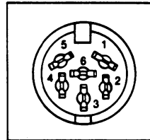
Figure 12-5. Serial Port Pinouts
