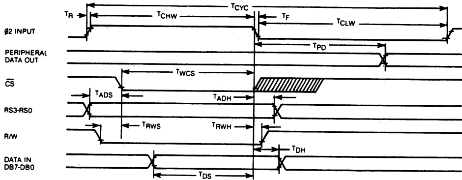
Figure 16-21. 6526 Write Timing Diagram
