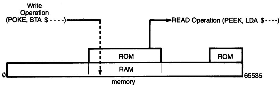
Figure 8-3. ROM Overlay
