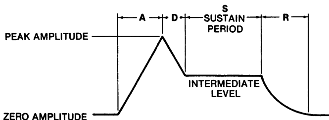
Figure 16-17. ADSR Envelope
