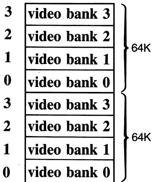
Figure 8-4. Video Banks within RAM Banks
