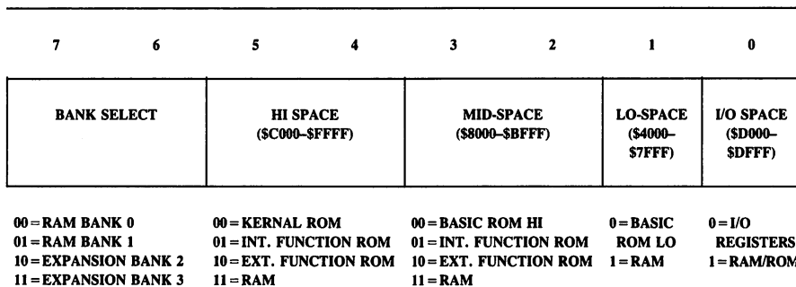
Figure 13-5. Configuration Register
