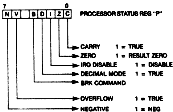
Figure 5-11. 8502 Status Register
