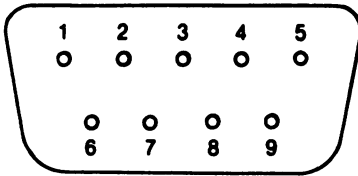
Figure 12-10. Controller Port Pinouts
