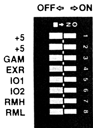
Figure 2 Port Switch
