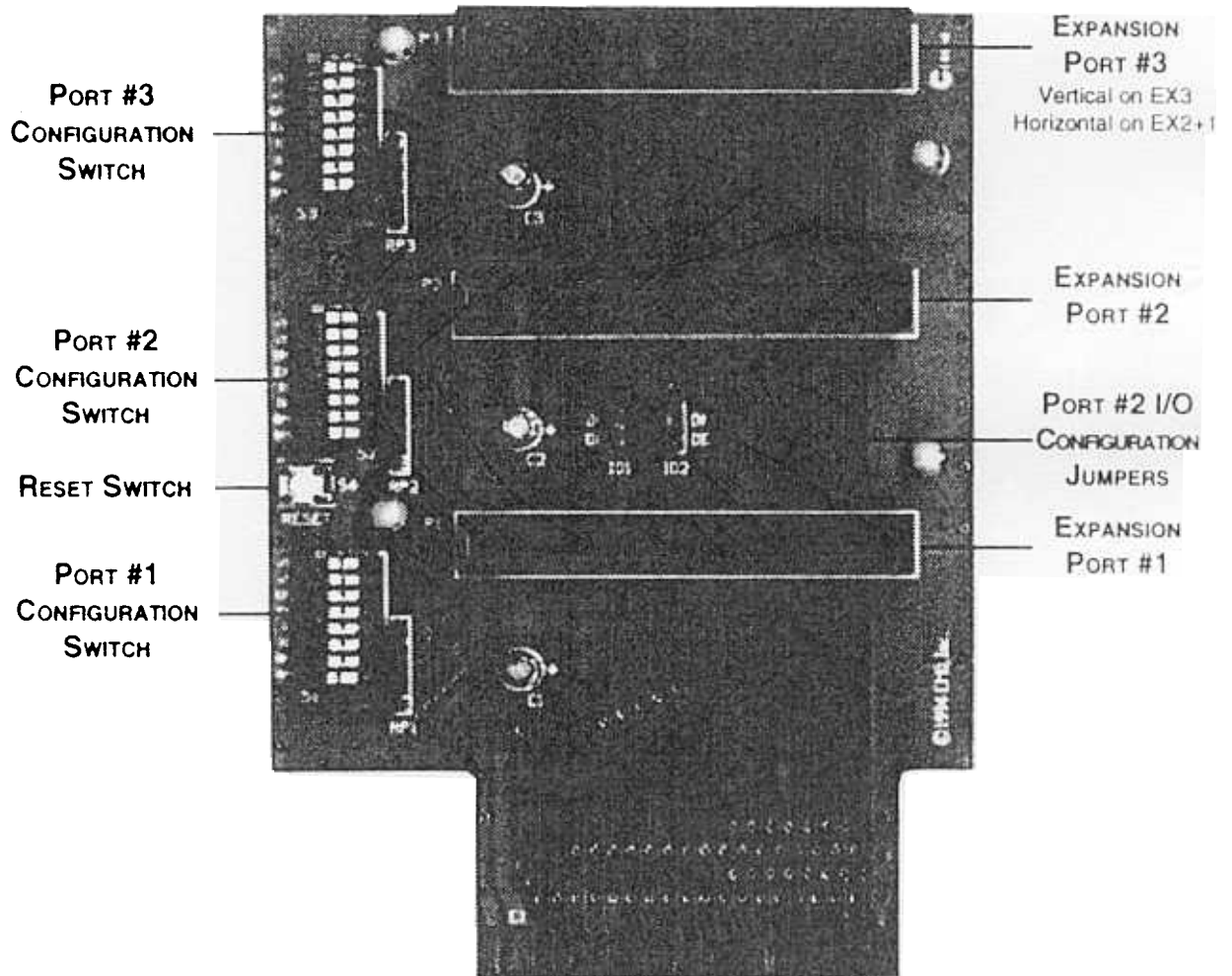
Figure 1 Top View of Cartridge Port Expander
