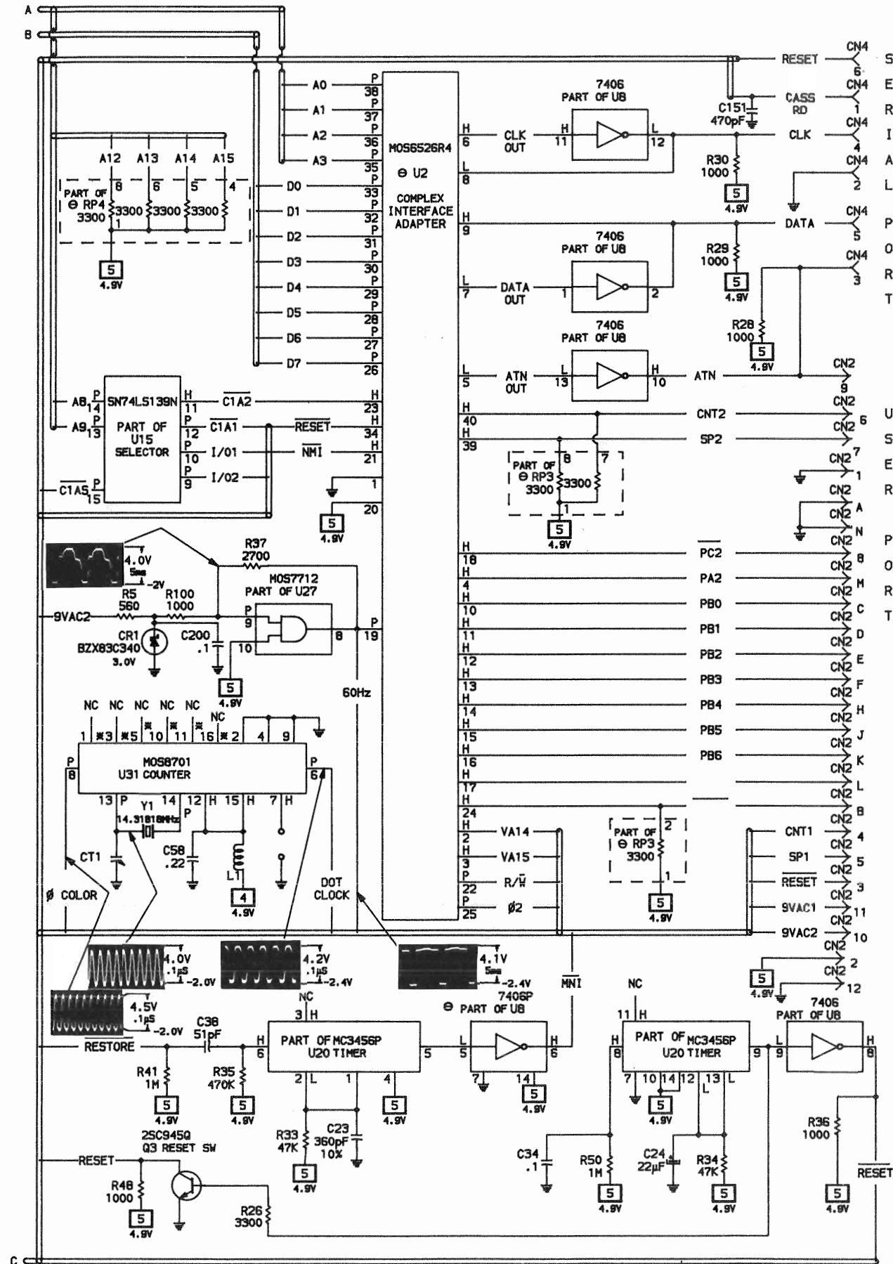
A PHOTOFACIT STANDARD NOTATION SCHEMATIC
