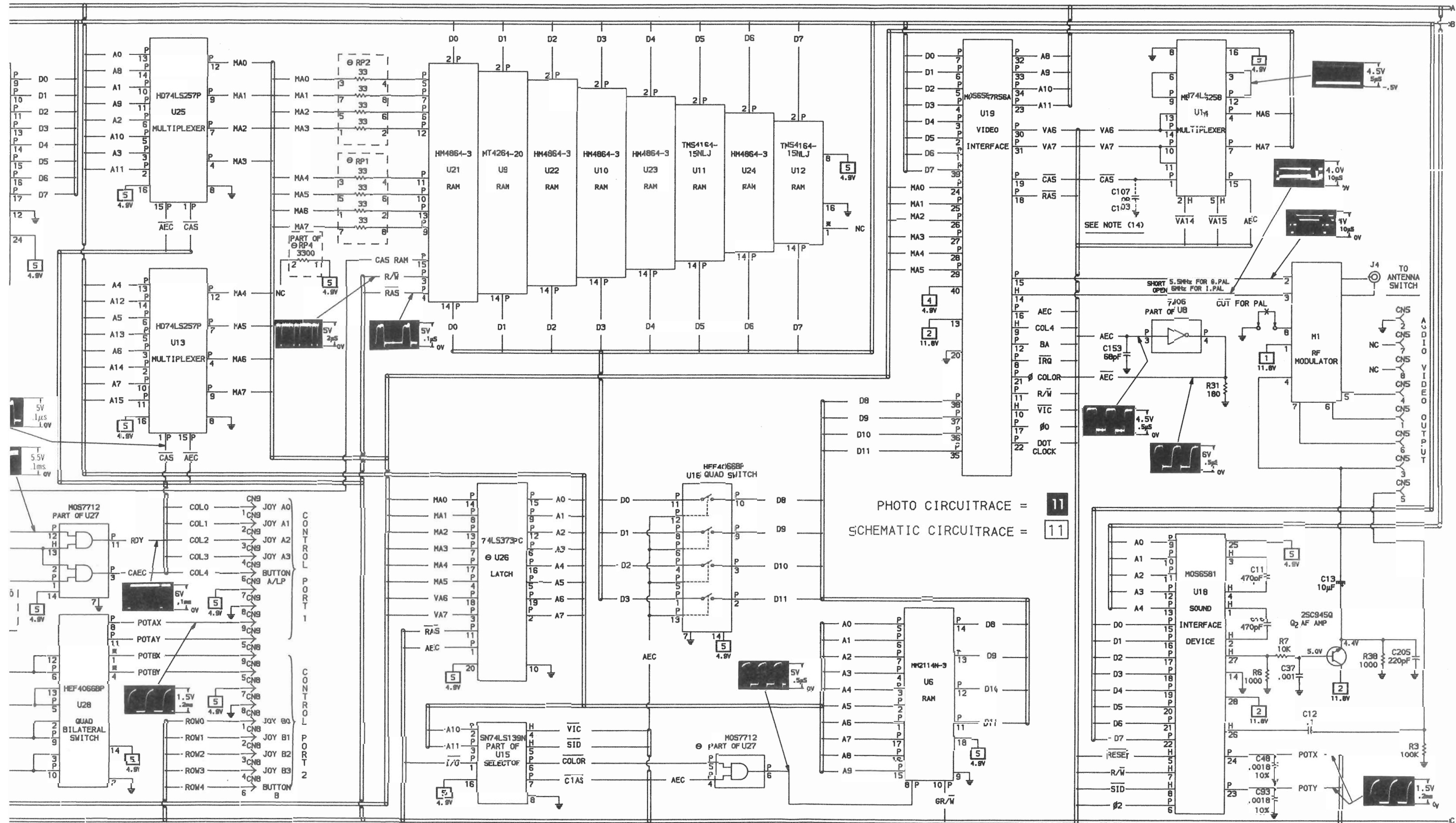
COMMODORE MODEL C64 (1984 VERSION)
